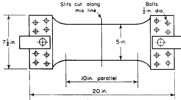
FIG. 2. Test panel.
